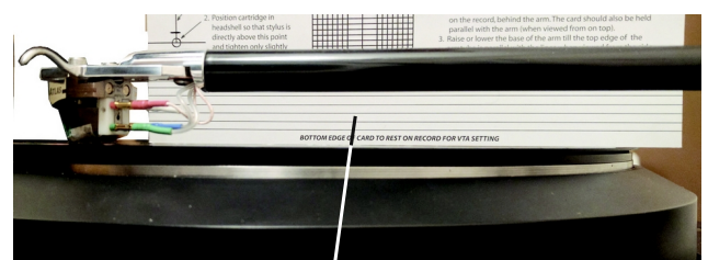
HORIZONTAL LINES ON ALIGNMENT GAUGE
