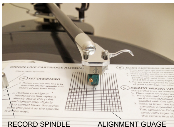
RECORD SPINDLE ALIGNMENT GAUGE
