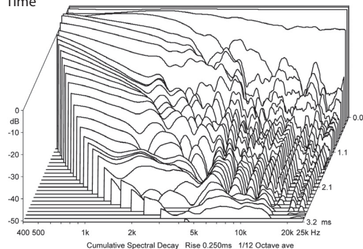
Magico S5 Mk II Waterfall: Energy Decay for Frequency and Time
